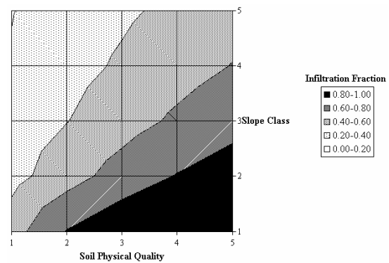
Figure 2. Infiltration fraction of a plot depending on slope and soil physical quality; slope is classified according to USLE ( 1: slope < 1%, 2: 1% ≤ slope < 3%, 3: 3% ≤ slope < 5%, 4: 5% ≤ slope < 20%, 5: slope > 20%); where soil physical quality represents its aggregate stability.
